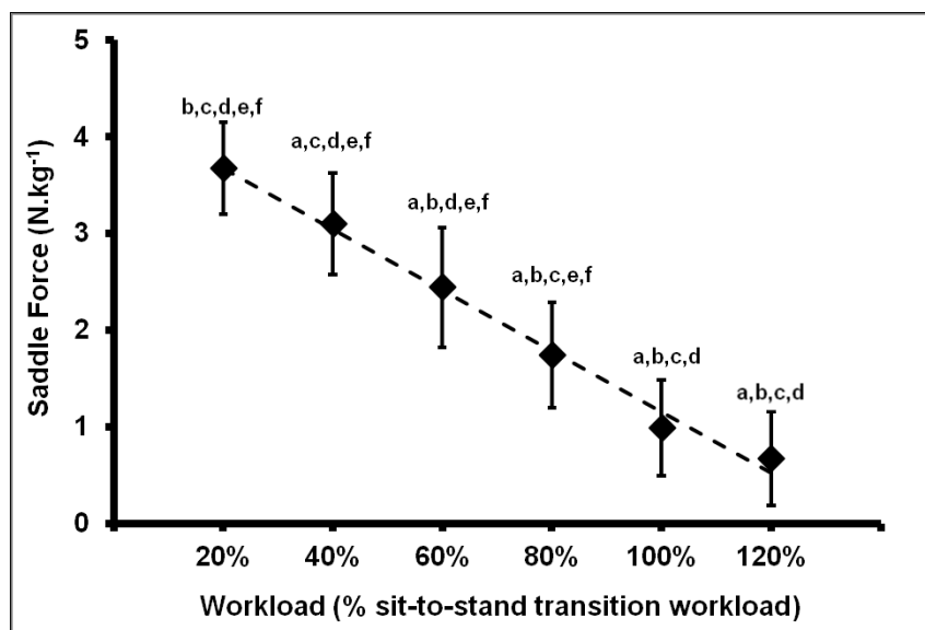
Figure 1: Minimum saddle vertical reaction force. a,b,c,d,e,f represent significant differences compared to 20, 40, 60, 80, 100, and 120% of SSTP, respectively.
