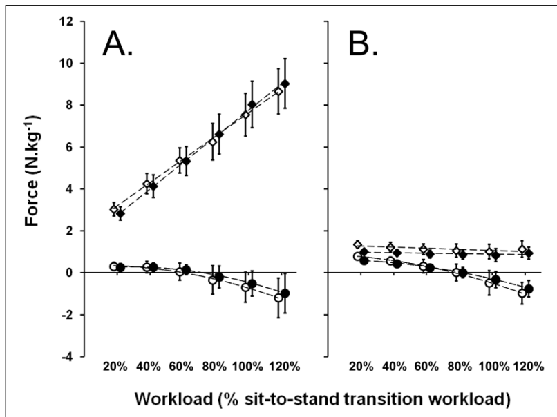
Figure 2: Minimum (dots) and maximum (diamonds) left (white), and right (black) vertical reaction forces. A. Pedals. B. Handlebars.
