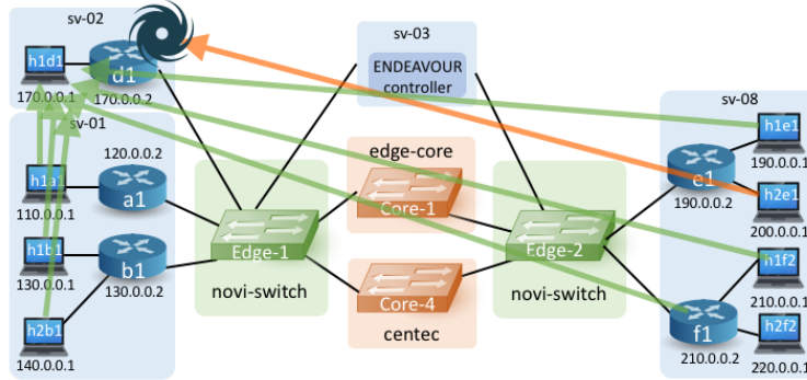
Figure 4: Blackholing topology
