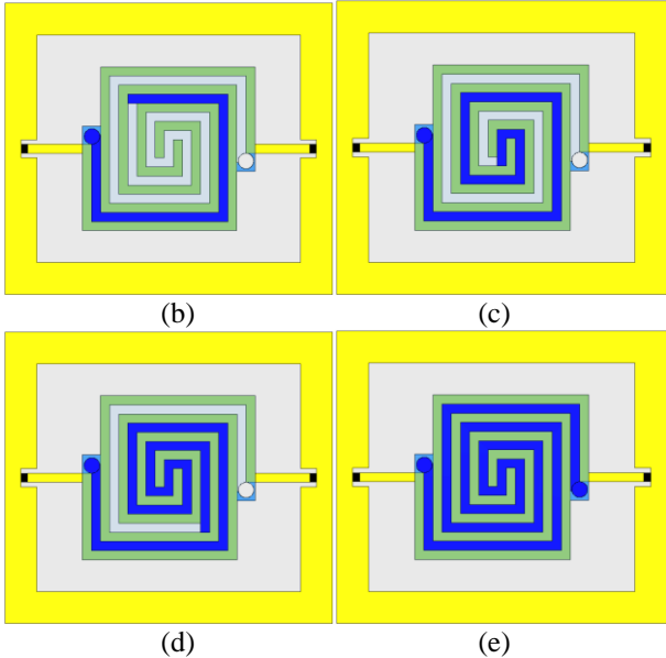
Figure 1: Design of the squared microfluidic capacitor: (a) 3D representation of the structure; fluid positions in channel: (b) POS1 (c) POS2 (d) POS3 (e) POS4.
