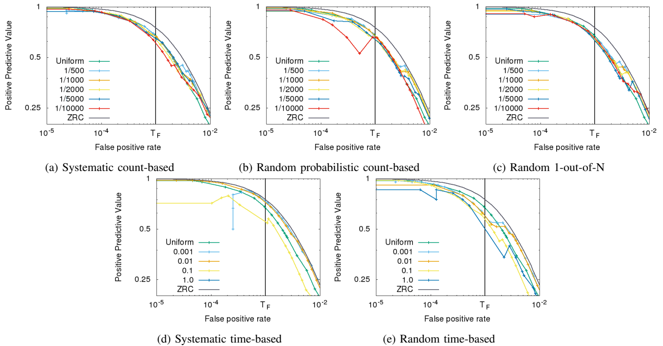
Fig. 3: IDS operation curves for the several sampling algorithms and multiple sampling rates.
