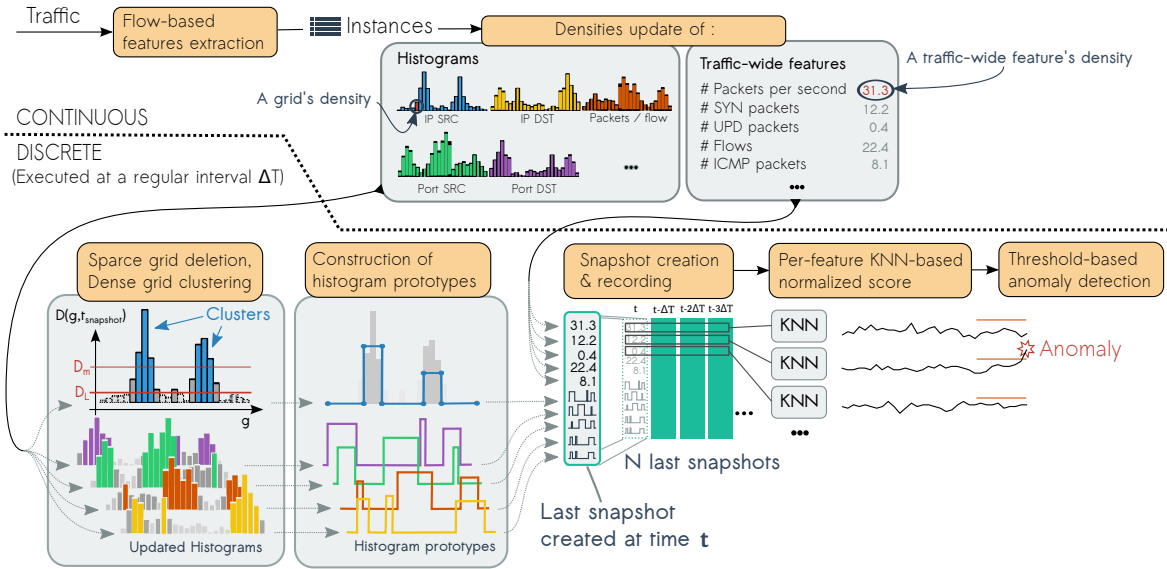
Fig. 1: An overview of the AATAC algorithm
