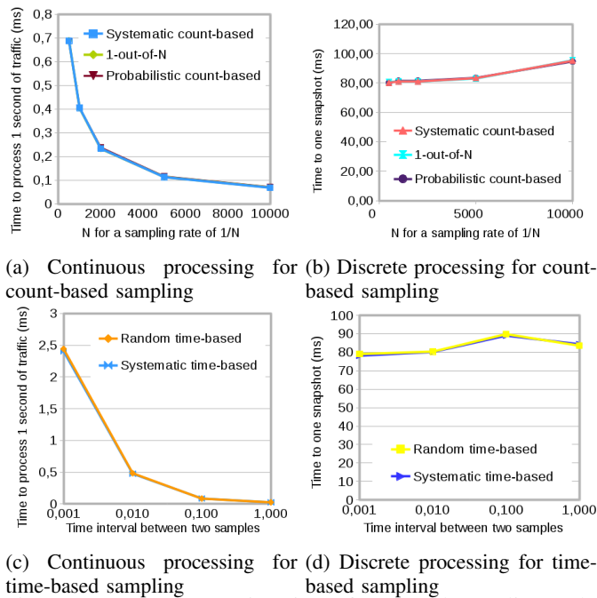
Fig. 4: AATAC's processing times for several sampling techniques and sampling rate
