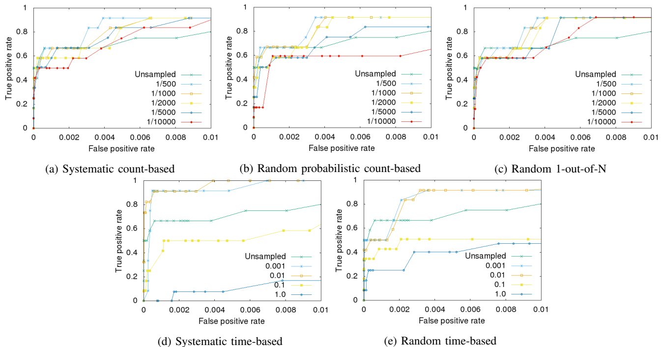
Fig. 2: ROC curves for the several sampling algorithms and multiple sampling rates.
