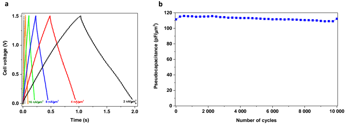
Figure 5. Galvanostatic charge/discharge measurements within a cell voltage of 1.5 V. (a) Even at very high current densities, from 2 to 64 nA/μm 2 (0.2 to 6.4 A/cm 2 ), the curves exhibit a symmetrical triangular profile with negligible IR-drop. (b) Capacitance retention under the severe operating conditions of 8 nA/μm 2 (0.8 A/cm 2 ) and 1.5 V.
