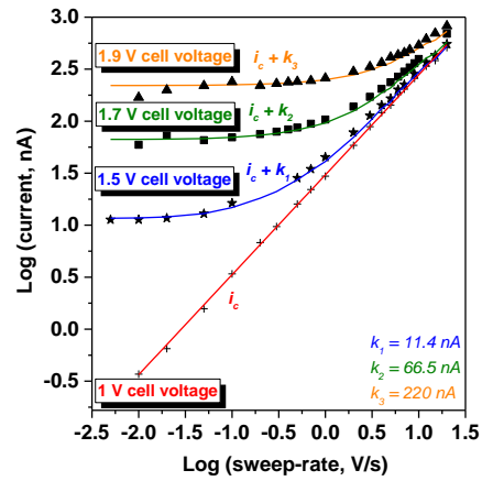
Figure 4. Sweep-rate dependence of the current of the nanosupercapacitor in de-aerated 0.5 M H 2 SO 4 at different cell voltages. At 1 V, the slope of the plot \log(i) vs. \log(v) is 0.96. Above 1 V, the experimental points are fitted by adding on the whole sweep-rate range a constant value k to the capacitive current i_c .
