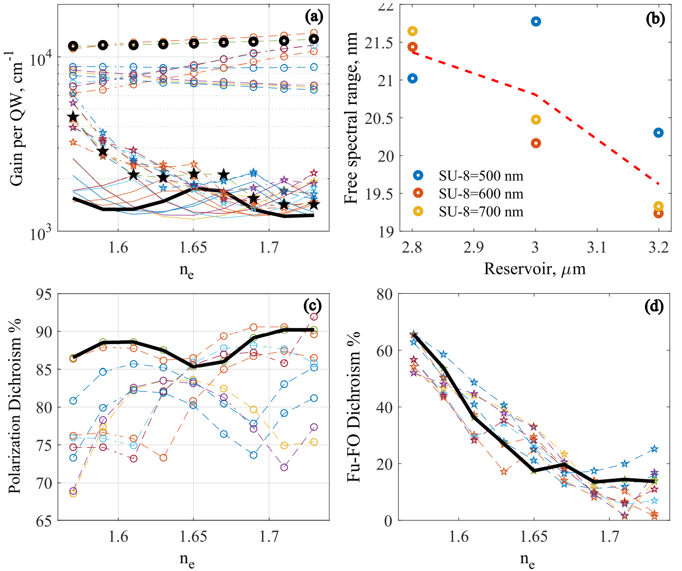
Fig. 11. Tuning performance ( n_e variation, plots a-c-d) at injection current of 5 mA for the 4\mu\text{m} oxide aperture; the nine investigated structures refer to the tolerance of reservoir ( 3.0 \pm 0.2\mu\text{m} ) and SU-8 ( 600 \pm 100\text{nm} ); in black, the nominal design. (a): modal losses for fundamental EM (continuous lines), fundamental OM (circles) and first order EM (stars). (c): polarization dichroism ( 1-G_{EM}/G_{OM} ). (d): dichroism, defined similarly to (c) but for G_{EM} and its corresponding first order mode. (b): free spectral range vs reservoir tolerance.
