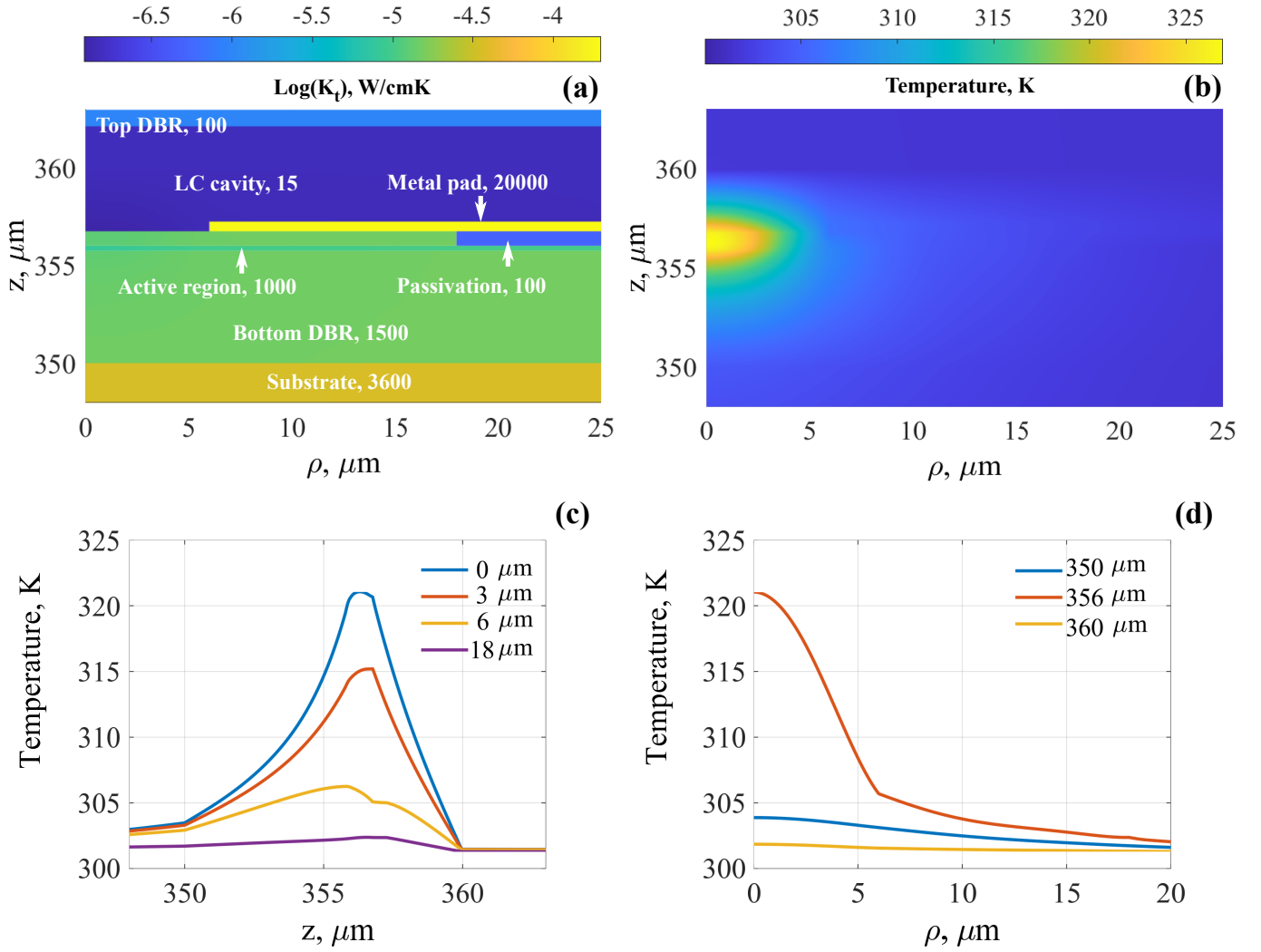
Fig. 9. (a) Map of the thermal conductivity ( \rho - z cut) and (b) corresponding thermal profile for a 4μm VCSEL with n_e = 1.63 and I=5 mA around the active region. Thermal conductivity values (in \text{W/cmK} ) are indicated by white labels, on the (a) map where the different regions are identified. For semiconductor see [33], for glass, top-DBR and for LC see [35]. (c) longitudinal temperature cuts at different radii (see legend); (d) transverse temperature cuts at different longitudinal sections. z=0 correspond to the heatsink, below the 350μm substrate.
