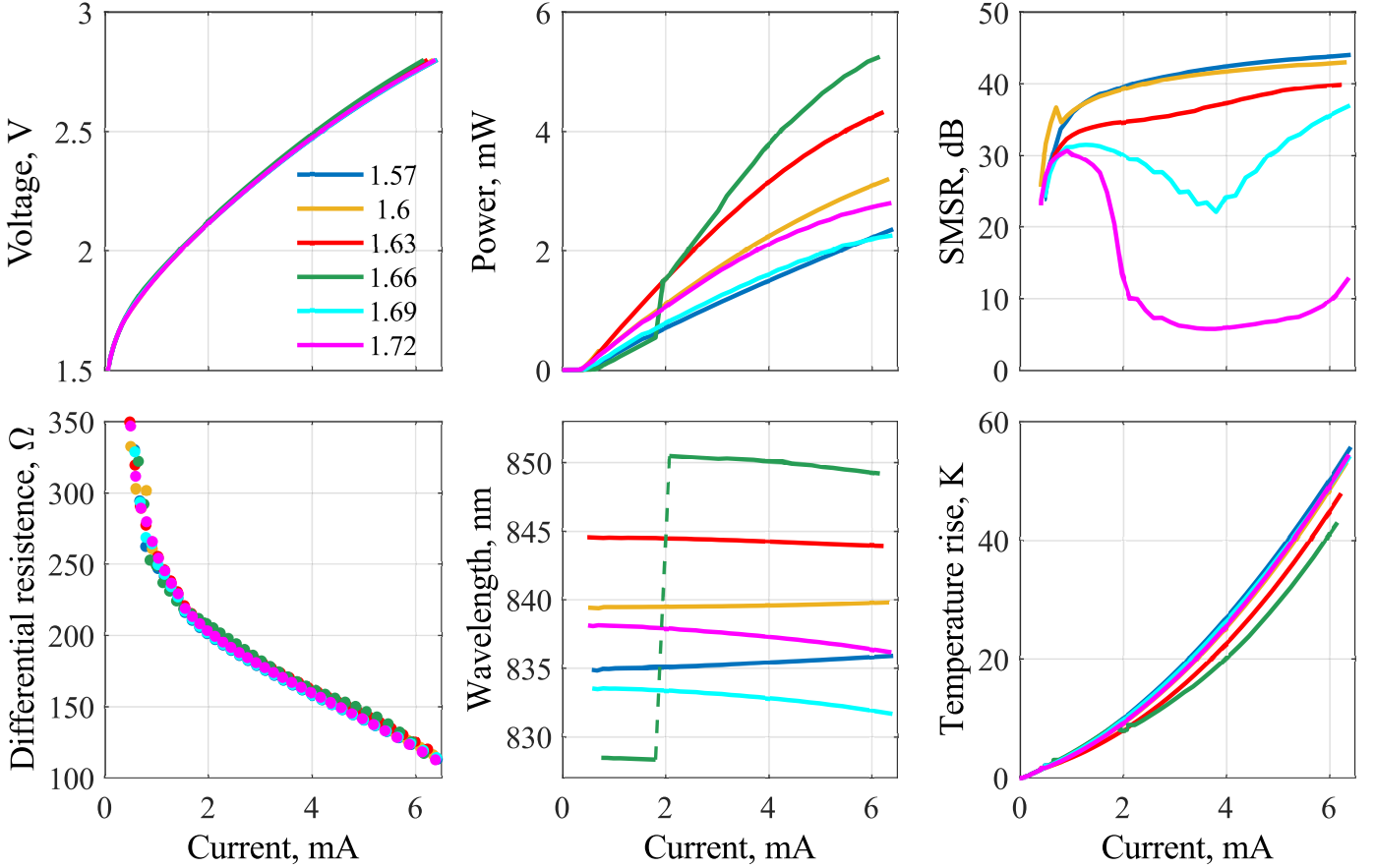
Fig. 8. Tuning performance ( n_e , see legend) for VI, LI, SMSR, differential resistance, lasing wavelength and peak temperature. A 4\mu\text{m} oxide apertures, 3\mu\text{m} reservoir at 600\text{ nm} SU-8 are considered, with an ambient temperature of 300\text{ K} .
