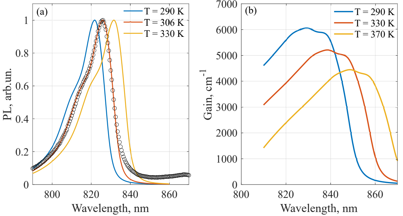
Fig. 2. (a): photoluminescence (PL) spectra at different temperatures; open black circles refer to the measured PL of a test sample. (b): gain spectra for different temperatures at n = p = 6 \times 10^{-12} \text{ cm}^{-2} .
