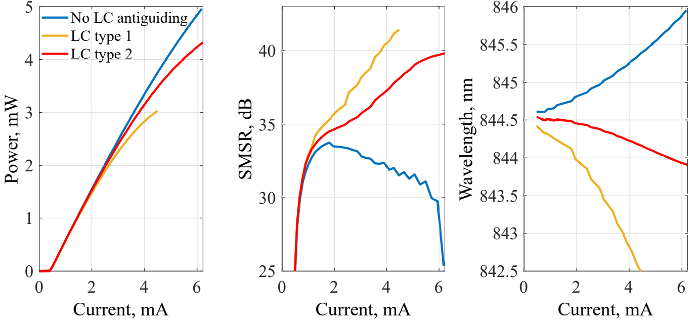
Fig. 10. LC-VCSEL performance vs. LC antiguiding features: LI, SMSR and lasing wavelength for a 4\mu\text{m} oxide aperture, n_e=1.63 , 3\mu\text{m} reservoir, 600 nm SU-8 and ambient temperature of 300 K.
