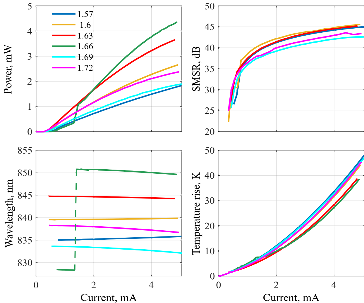
Fig. 13. Tuning performance ( n_e legend) of a 3 \mu\text{m} oxide aperture LC-VCSEL. 3 \mu\text{m} reservoir and 600 nm SU-8 are considered, with an ambient temperature of 300 K.
