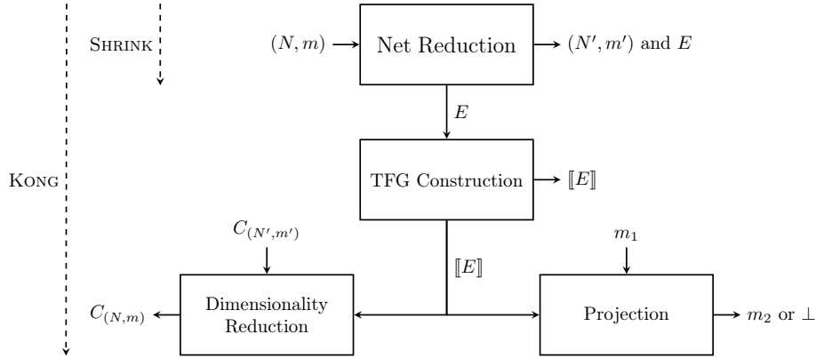
Fig. 1: KONG’s architecture.
