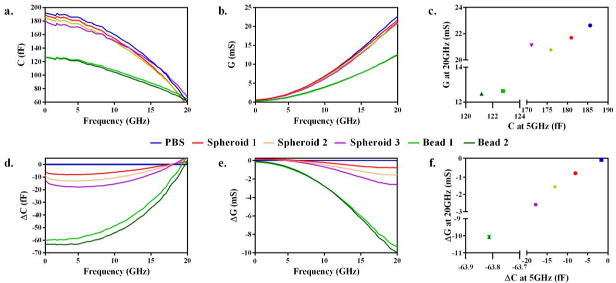
Figure 4: Measurements performed with different polystyrene beads and spheroids. Extracted (a) capacitance and (b) conductance obtained for the different objects. (c) Complex electrical representation of the capacitance and conductance, at 5 GHz and 20 GHz respectively. (d) Capacitive and (e) conductive contrasts. (f) Complex electrical representation of the capacitive and the conductive contrasts at 5 GHz and 20 GHz respectively. The tested spheroids and polystyrene beads present diameters between 200\mu\text{m} and 360\mu\text{m} .
