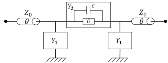
Figure 3: Electrical model of the device.
