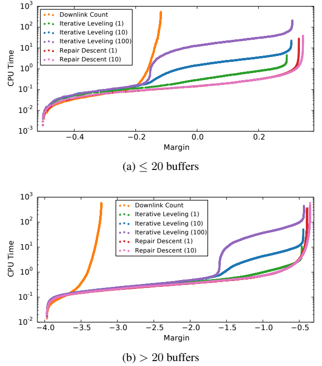
Figure 2: Comparison with the state of the art on synthetic scenarios.
